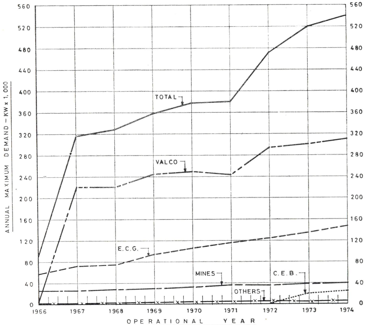
POWER PRODUCTION STATISTICS ANNUAL MAXIMUM DEMAND IN KW
