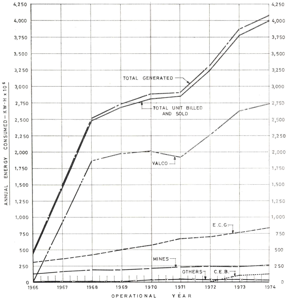
ANNUAL ENERGY CONSUMED PER CLASS OF CUSTOMER IN 10 3 KWH
